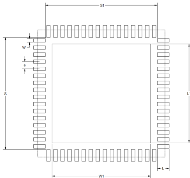
Figure 6.1. PCB Land Pattern
